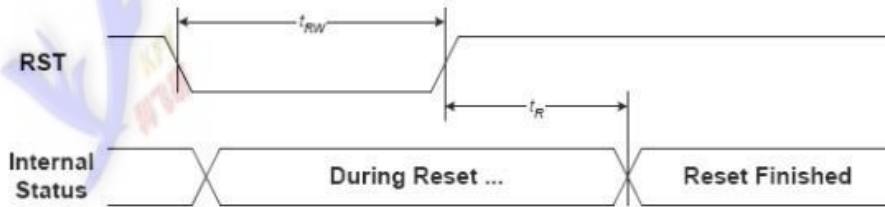
FIGURE 15: Reset Characteristics
