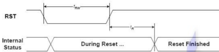
FIGURE 15: Reset Characteristics
